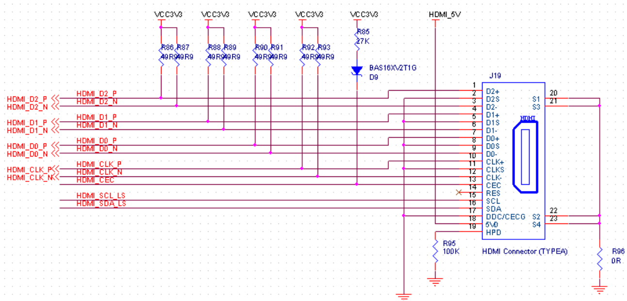
Figure 3-8-1: Design schematic of HDMI interface
