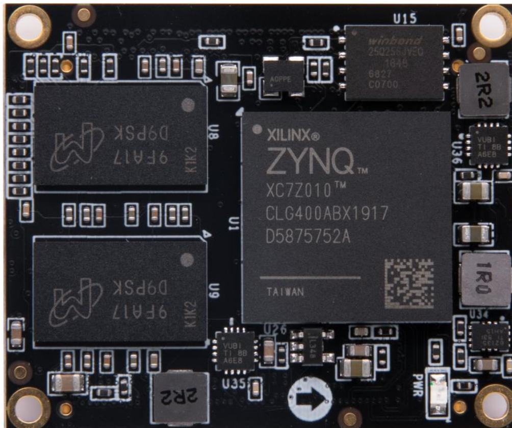
AC7Z010 Core Board Front View
