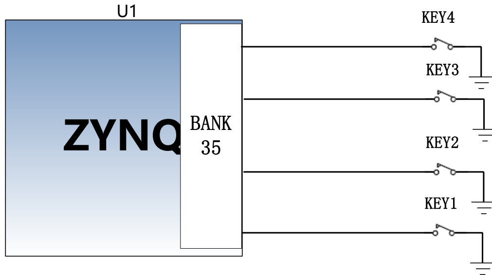
Figure 3-16-1: User key connection diagram
