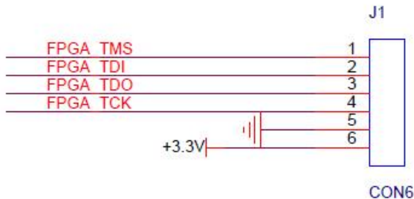
JTAG Interface Schematic
