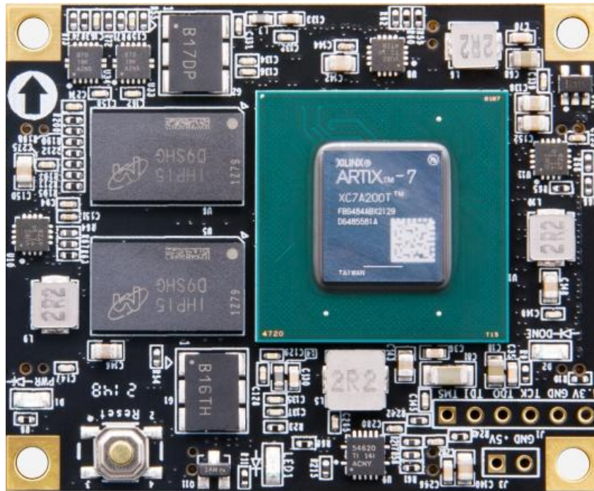
AC7200 Core Board (Front View)
