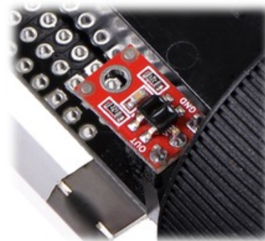
Close-up of QTR-1RC reflectance sensor connected to a Zumo shield via a 1×3 female header.
