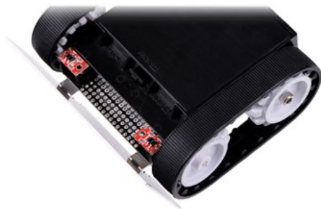
Zumo robot with QTR-1RC reflectance sensors.
