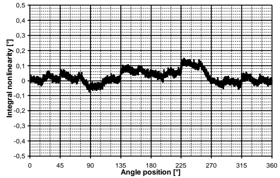
Fig. 26: Typical integral nonlinearity at optimal parameters
