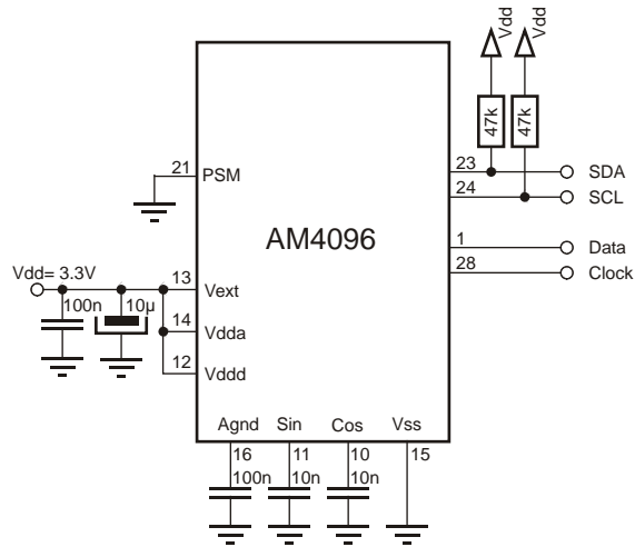
Fig. 34: Application scheme for autonomous power save mode
