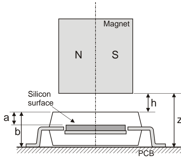
Fig. 31: AM4096 and the magnet with dimensions
