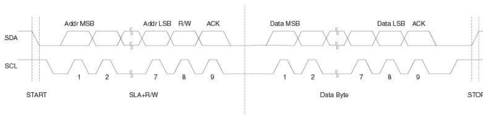
Fig. 5: TWI Address and Data Packet Format
