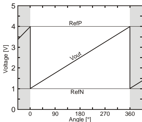
Fig. 18: One period per revolution (“Dac”= 0 0)
