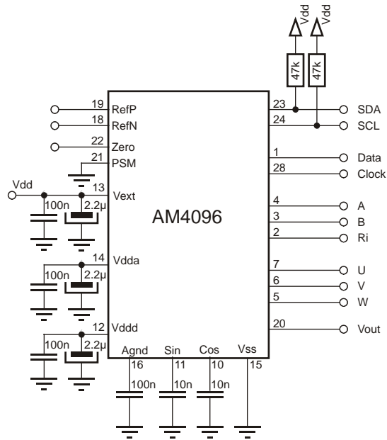
Fig. 33: Typical application scheme
