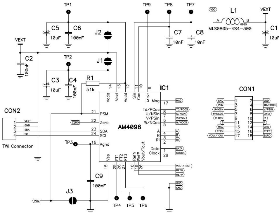
Fig. 36: RMK4 with schematic
