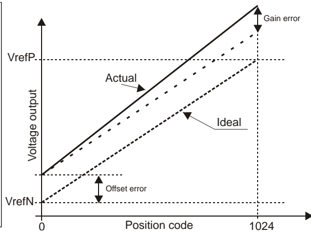
Fig. 23: Offset and Gain error of the DAC
