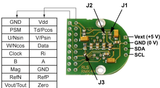
Fig. 36: RMK4 with schematic
