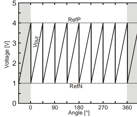
Fig. 21: Eight periods per revolution (“Dac”= 1 1)
