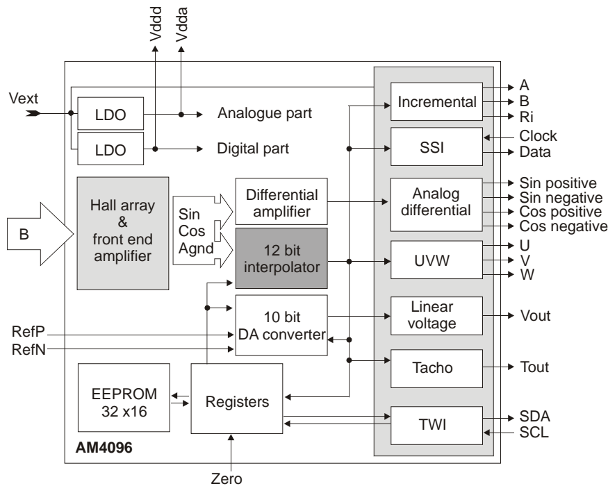
Fig. 2: AM4096 block diagram
