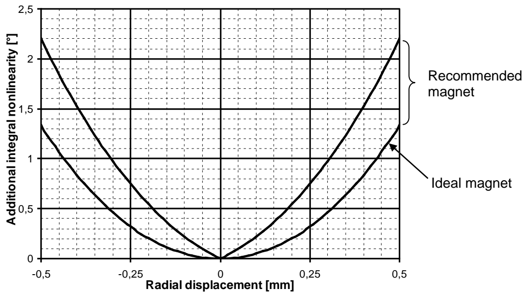
Fig. 30: Additional integral nonlinearity error caused by magnet displacement
