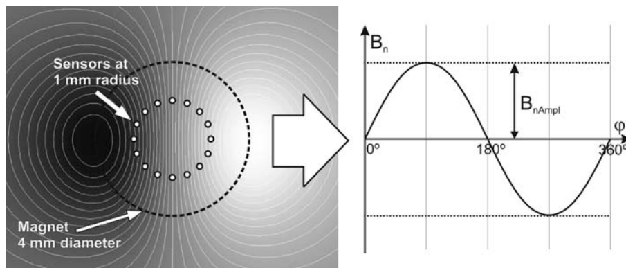
Fig. 28: Distribution of B_n and its modulation if the magnet is rotated through 360°
