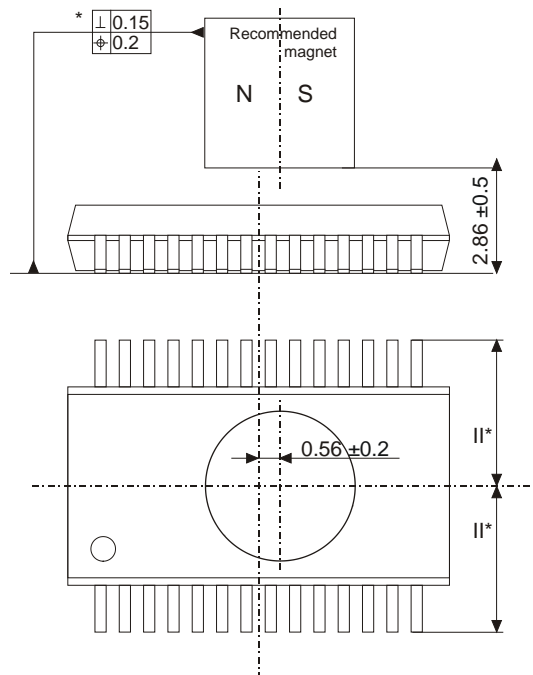
Fig. 32: Mounting instructions
