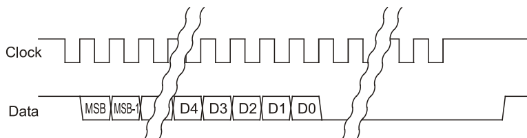
Fig. 14: SSI single read, SSlref is set to 00
