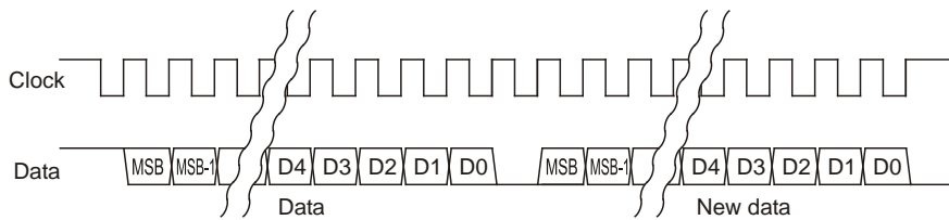
Fig. 16: SSI fast position read, SSlref is set to 11
