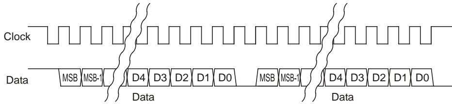
Fig. 15: SSI multi-read of the same position data, “SSlref” is set to 10
