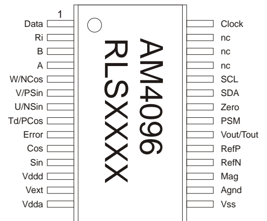
Fig. 3: Pin description for AM4096
