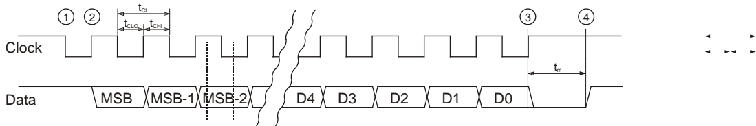
Fig. 13: SSI timing diagram with monoflop timeout
