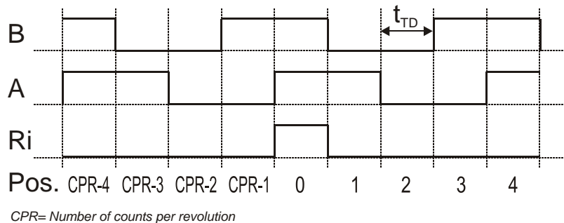
Fig. 12: Timing diagram for incremental output
