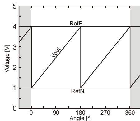
Fig. 19: Two periods per revolution (“Dac”= 0 1)
