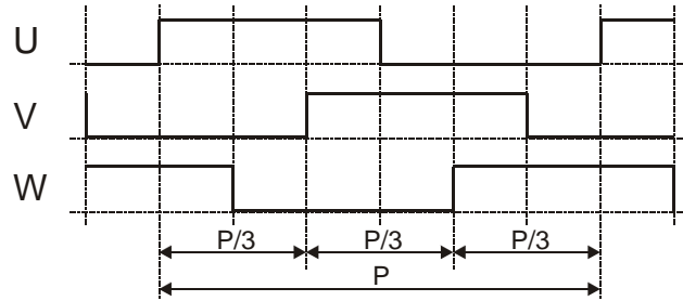
Fig. 17: UVW timing diagram for CW magnet rotation
