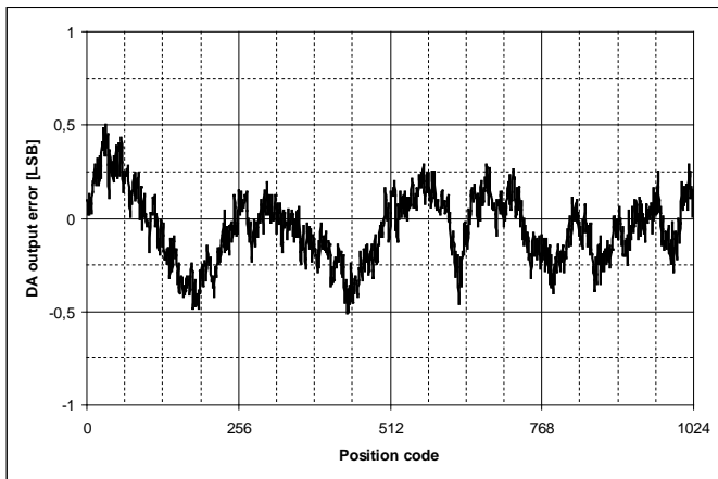
Fig. 22: Typical relative accuracy plot of the DAC
