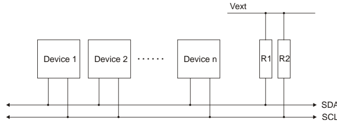
Fig. 4: TWI bus interconnection
