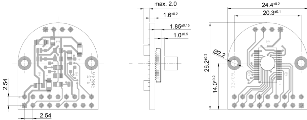
Fig. 35: RMK4 installation drawing
