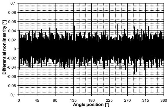
Fig. 25: Typical differential nonlinearity
