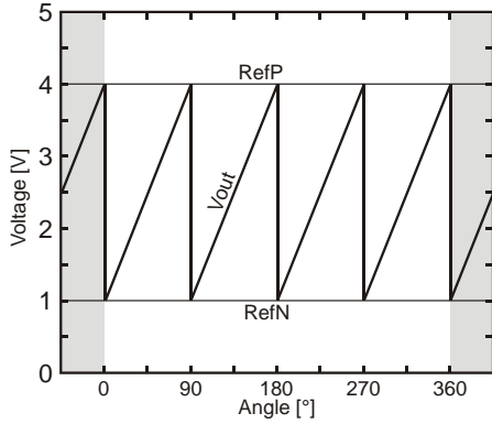
Fig. 20: Four periods per revolution (“Dac”= 1 0)
