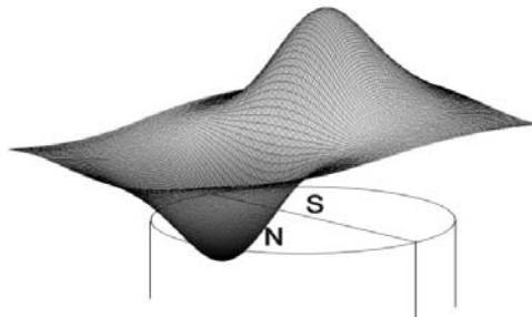
Fig. 27: Distribution of the perpendicular component of B
