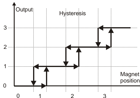
Fig. 24: Hysteresis
