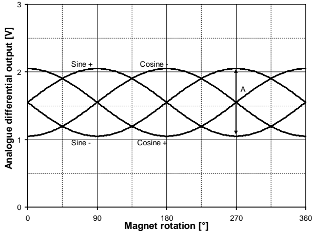
Fig. 11: Timing diagram for differential analogue output
